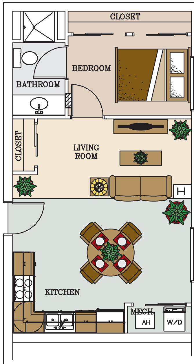
APARTMENT TYPE-B 1 BEDROOM 528 SQ. FT.
